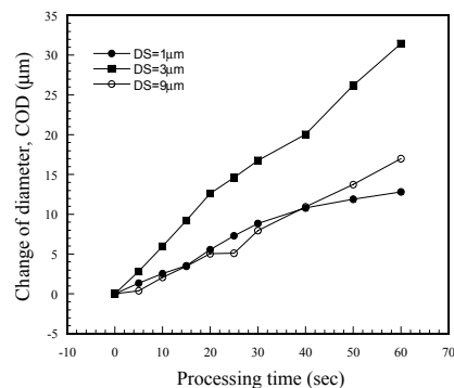
Fig. 7. Variations of micro-diameter vs. processing time. (Frequency: 12 Hz, Diamond grain size: 1 \mu\text{m} , 3 \mu\text{m} , 9 \mu\text{m} )
