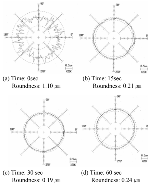
(A) Changes in roundness. (Frequency: 0 Hz, Diamond grain size: 1 \mu\text{m} , Processing time: 60 sec)
