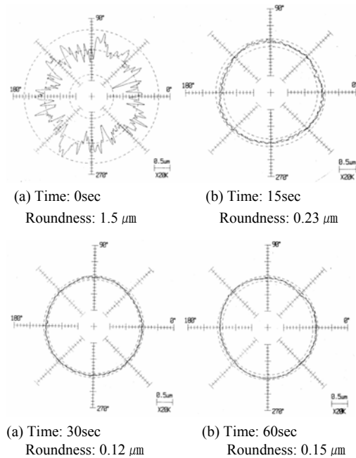
(B) Changes in roundness. (Frequency: 12 Hz, Diamond grain size: 1 \mu\text{m} , Processing time: 60 sec)
