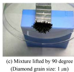
Fig. 5. Photographs of mechanical mixture of unbonded type magnetic abrasives.
