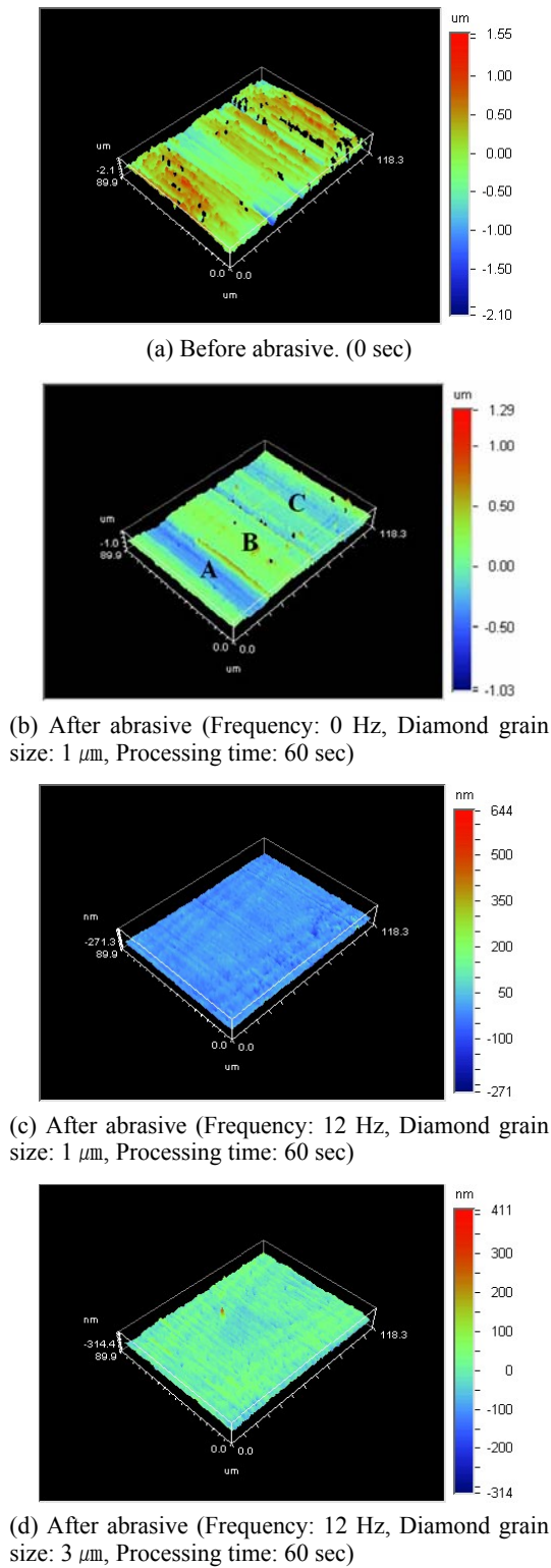
Fig. 11. Three dimensional surface conditions before and after processing.
